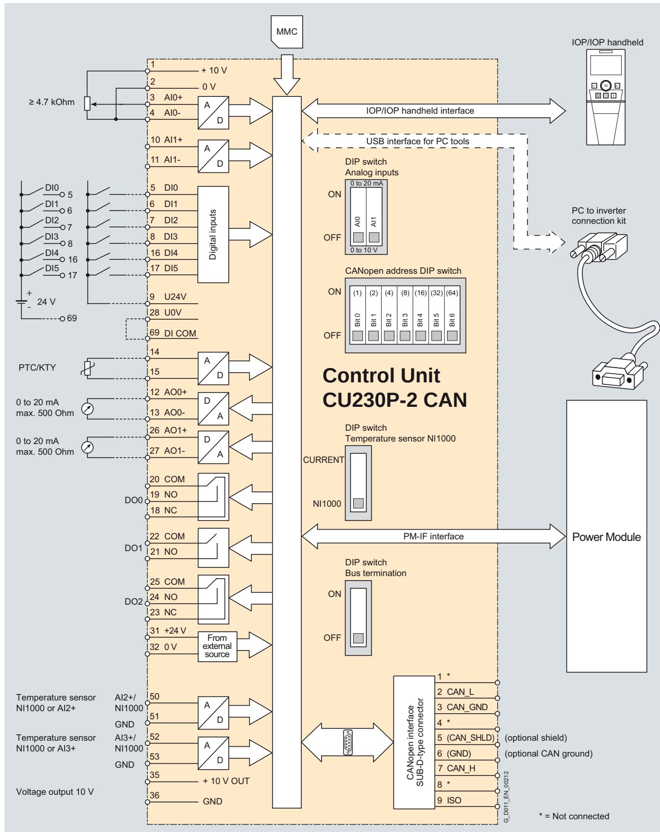
CU230P-2 CAN Control Unit connection diagram
