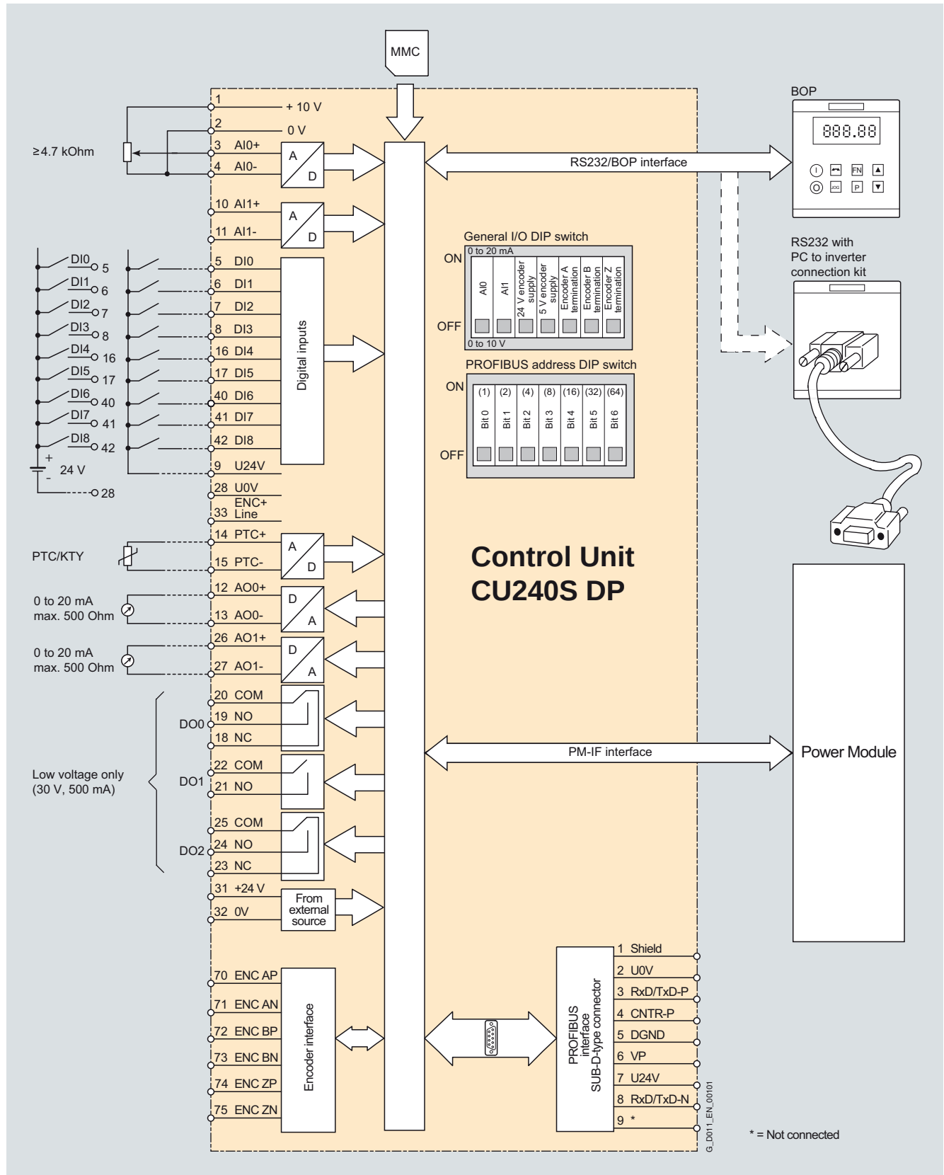
CU240S DP Control Unit connection diagram
