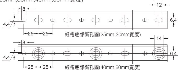
綫槽底部衝孔圖(25mm,30mm,40mm,60mm寬度)
